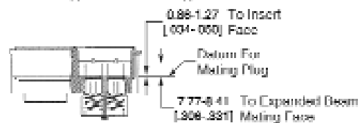
Section Z-Z
