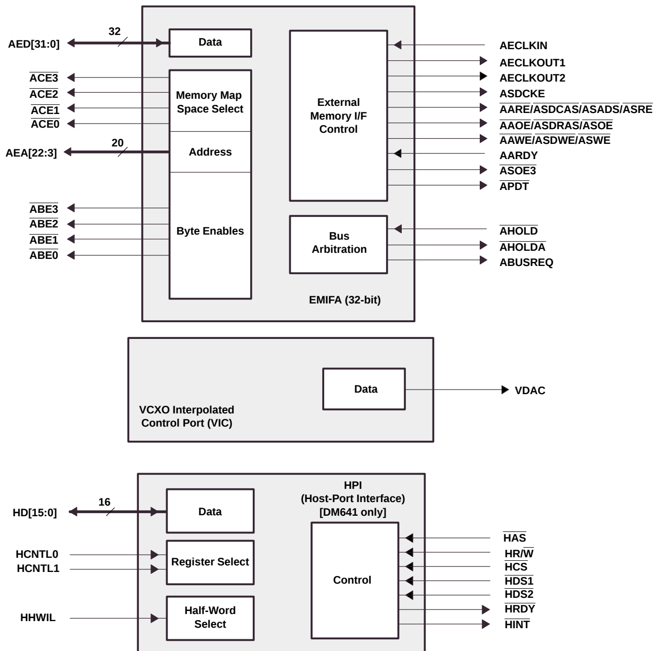
Figure 1–6. Peripheral Signals
