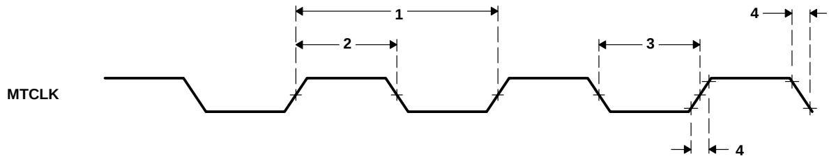
Figure 17–2. MTCLK Timing (EMAC – Transmit)
