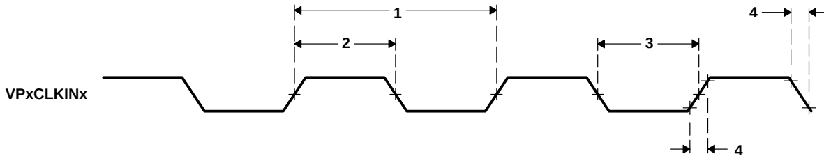
Figure 16–1. Video Port Capture VPxCLKINx Timing
