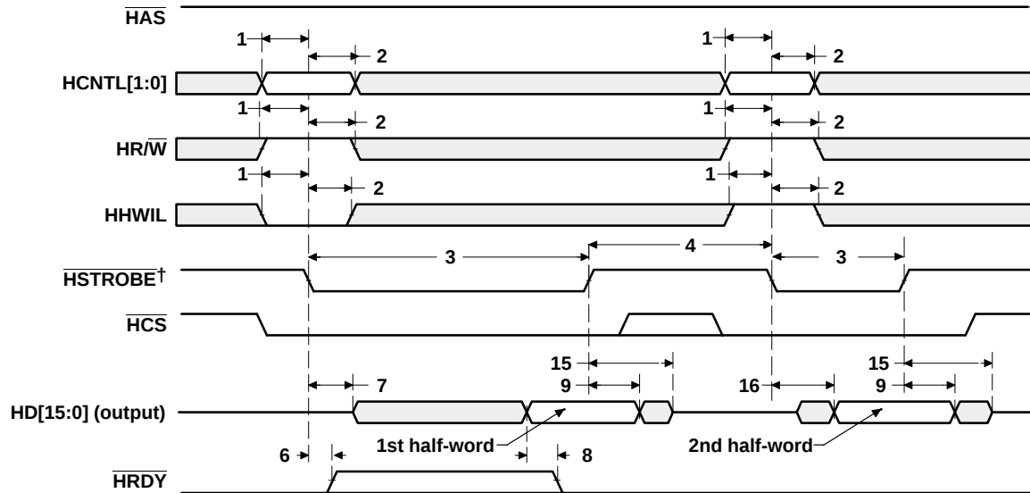
Figure 14-1. HPI16 Read Timing ( \overline{HAS} Not Used, Tied High) [for DM641 Only]
