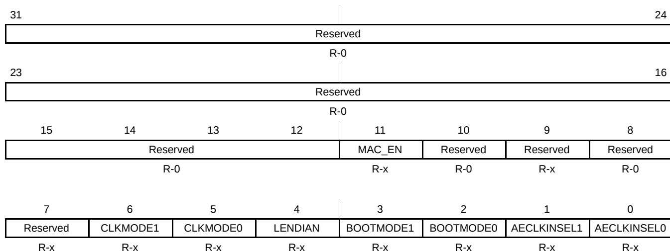
Figure 2–4. Device Status Register (DEVSTAT) Description – 0x01B3 F004
