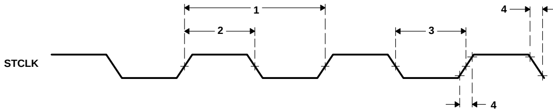
Figure 16–2. STCLK Timing
