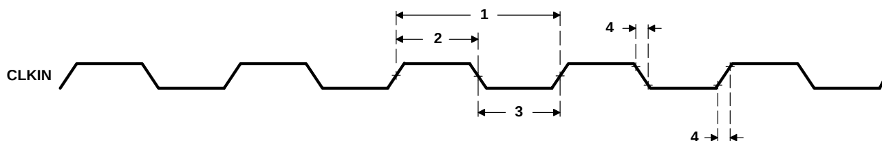
Figure 4–1. CLKIN Timing
