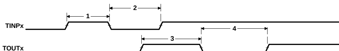
Figure 19–1. Timer Timing
