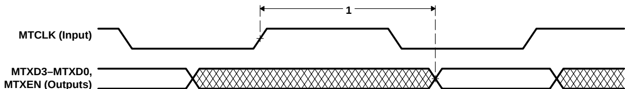
Figure 17–4. EMAC Transmit Interface Timing
