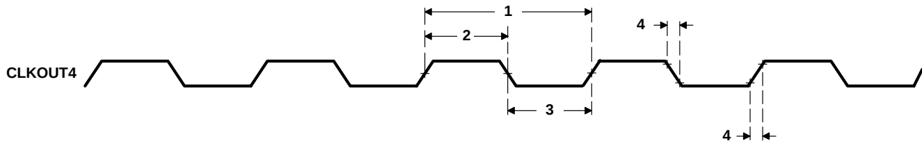
Figure 4–2. CLKOUT4 Timing
