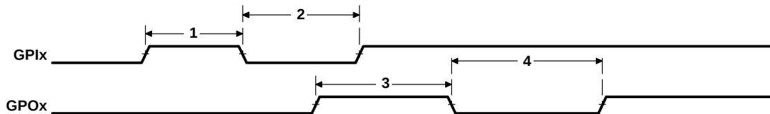
Figure 20–1. GPIO Port Timing
