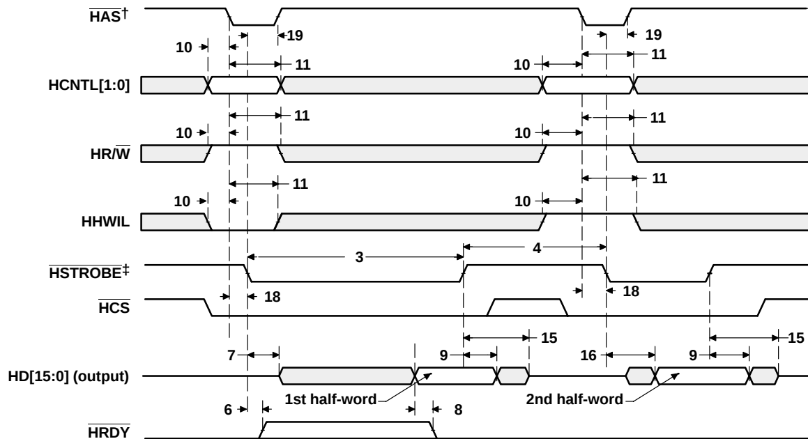
Figure 14-2. HPI16 Read Timing ( \overline{HAS} Used) [for DM641 Only]
