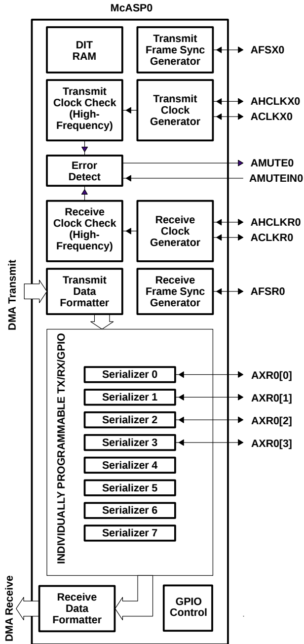
Figure 2-12. McASP0 Configuration
