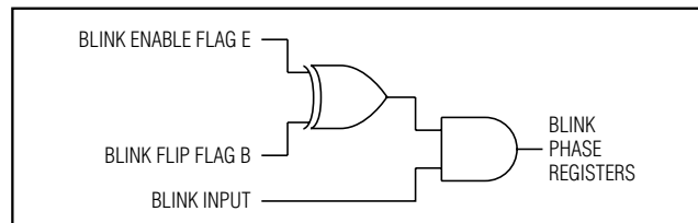
Figure 11. Blink Logic
