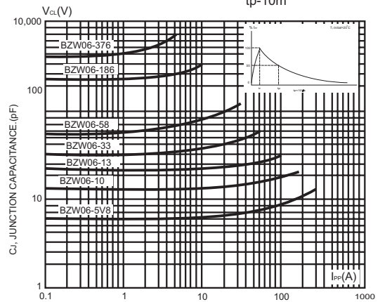
FIG.4- CLAMPING VOLTAGE VERSUS PEAK PULSE CURRENT. EXponential WAVEFORM t_p=200\mu s t_p=1ms t_p=10m
