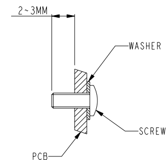
DETAIL 2 RECOMMENDED SCREW LENGTH
