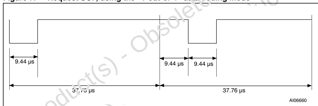
Figure 8. Request EOF
