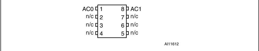
Figure 2. UDFPN8 connections
