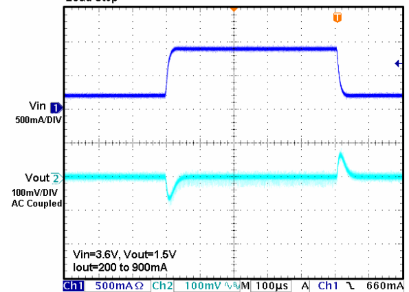
Load Step
