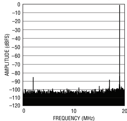
LTC2264-14: 8k Point FFT, f_{IN} = 139\text{MHz} , -1\text{dBFS} , 40Msps
