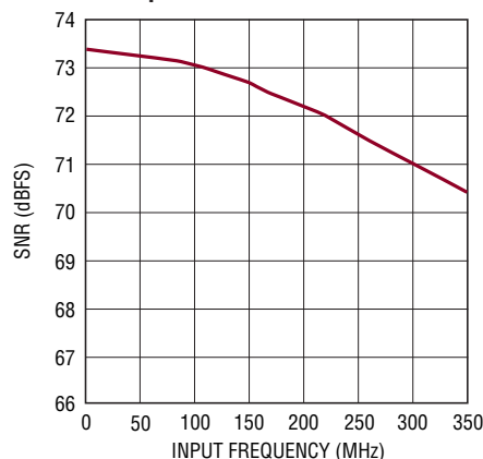
LTC2264-14: SNR vs Input Frequency, -1\text{dBFS} , 2V Range, 40Msps
