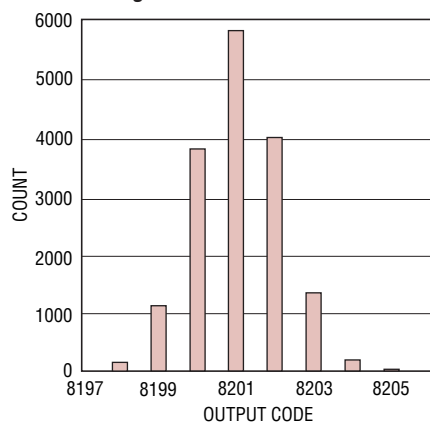
LTC2265-14: Shorted Input Histogram
