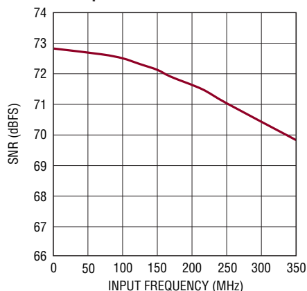
LTC2263-14: SNR vs Input Frequency, -1dBFS, 2V Range, 25Mps
