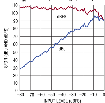
LTC2264-14: SFDR vs Input Level, f_{IN} = 70\text{MHz} , 2V Range, 40Msps
