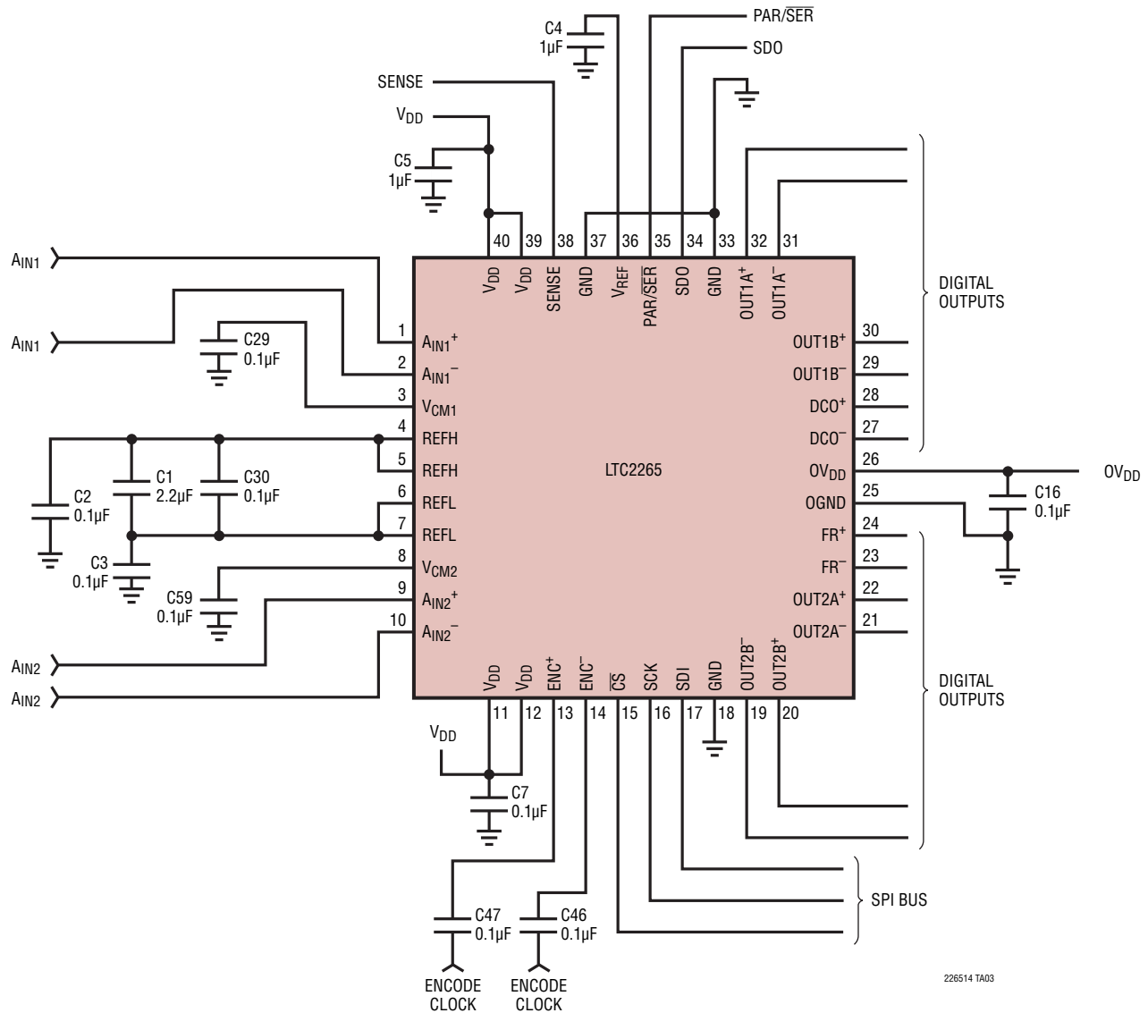
LTC2265 Schematic
