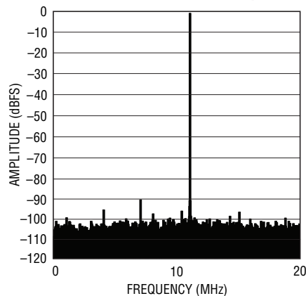
LTC2264-14: 8k Point FFT, f_{IN} = 69\text{MHz} , -1\text{dBFS} , 40Msps
