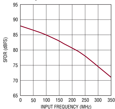
LTC2263-14: SFDR vs Input Frequency, -1dBFS, 2V Range, 25Mps
