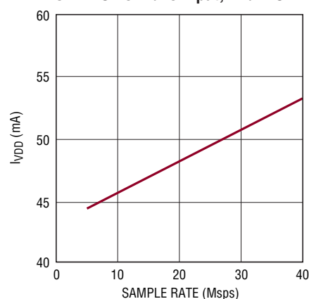
LTC2264-14: I_{VDD} vs Sample Rate, 5MHz Sine Wave Input, -1\text{dBFS}
