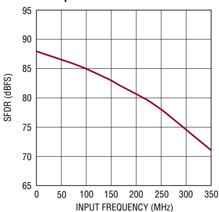
LTC2264-14: SFDR vs Input Frequency, -1\text{dBFS} , 2V Range, 40Msps
