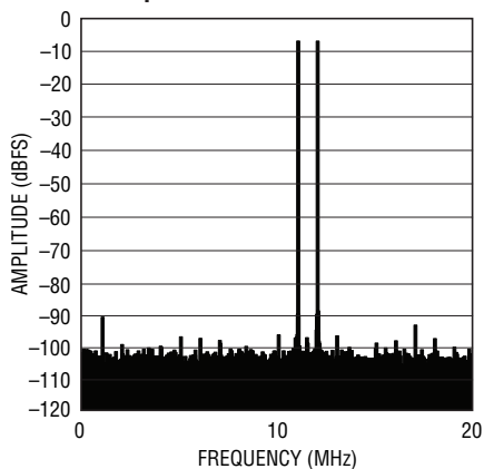
LTC2264-14: 8k Point 2-Tone FFT, f_{IN} = 68\text{MHz} , 69\text{MHz} , -1\text{dBFS} , 40Msps
