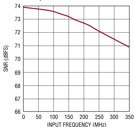
LTC2265-14: SNR vs Input Frequency, -1\text{dBFS} , 2\text{V} Range, 65\text{Mpsps}
