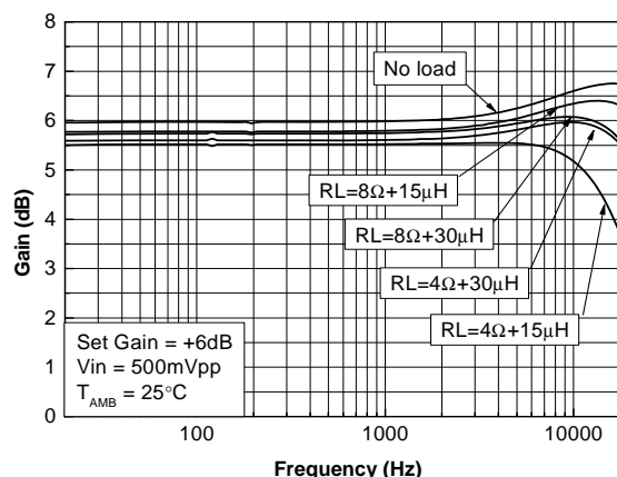
Figure 36. Gain vs. frequency @ +6 dB gain
