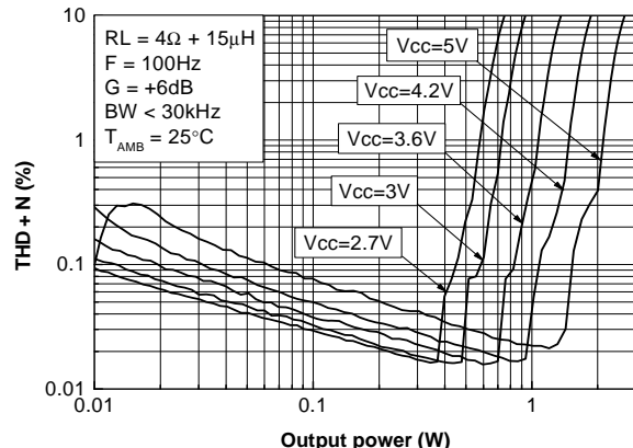
Figure 16. THD+N vs. output power @ 4 \Omega and 100 Hz
