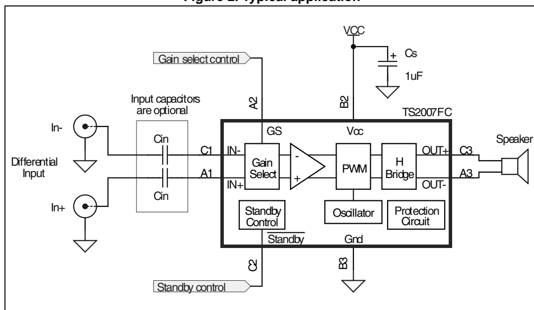
Figure 2. Typical application
