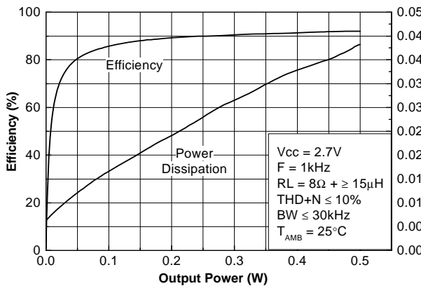
Figure 13. Efficiency vs. output power @ 2.7 V and 8 \Omega
