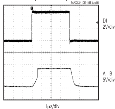
DRIVER PROPAGATION (250kbps) (MAX13412E)
