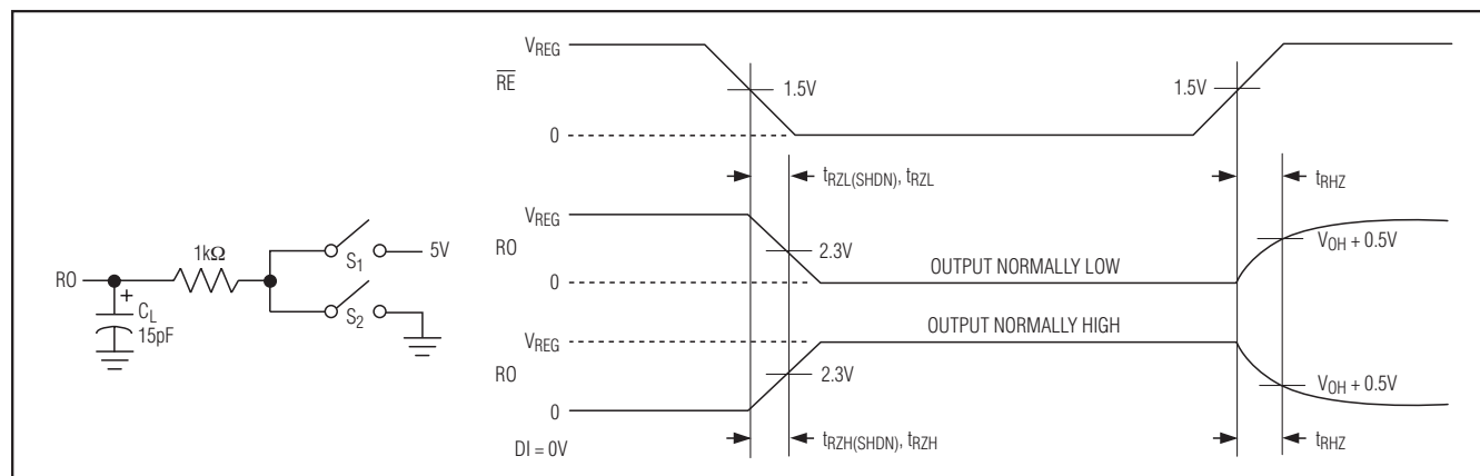
Figure 7. Receiver Enable and Disable Times
