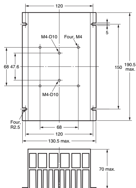
Mounting Holes
