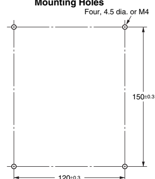
Mounting Holes
