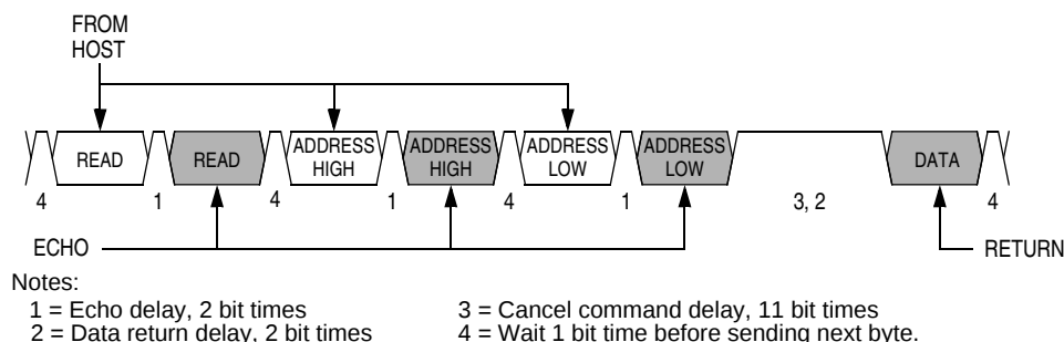
Figure 13-10. Read Transaction
