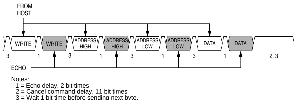
Figure 13-11. Write Transaction
