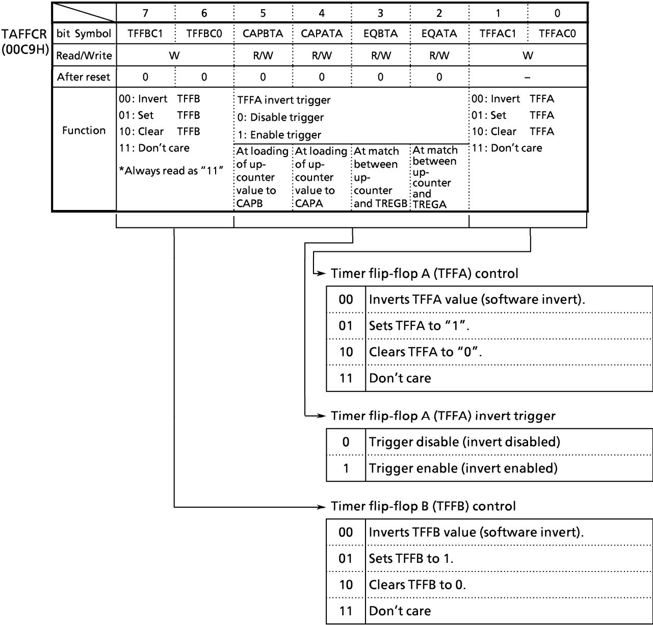
Figure 3.9 (16) 16-Bit Timer A F/F Control (TAFFCR)
