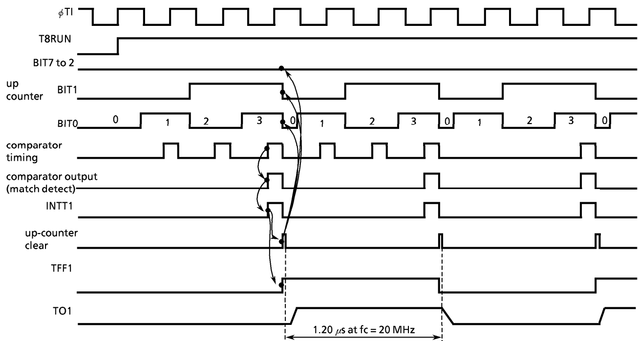
Figure 3.8 (11) Square Wave (50% Duty) Output Timing Chart
