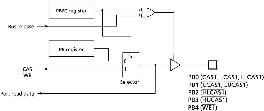
Figure 3.5 (11) Port B
