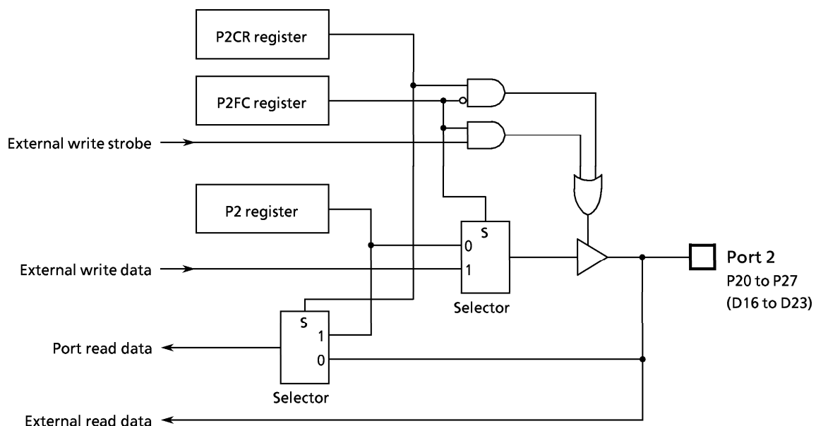
Figure 3.5 (3) Port 2
