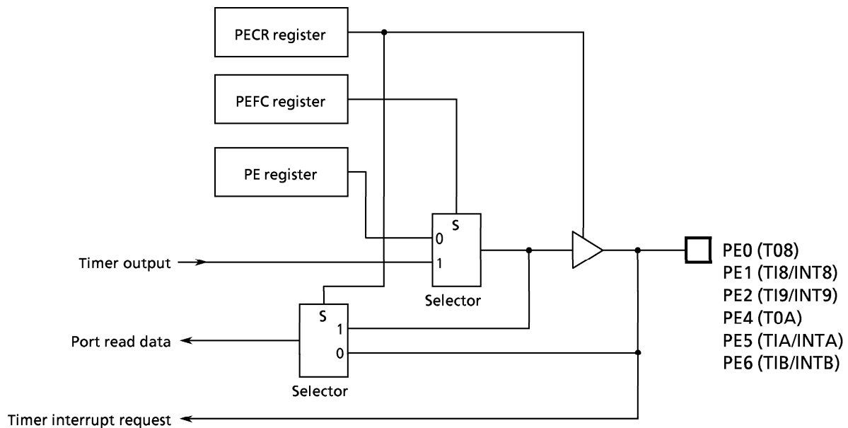
Figure 3.5 (14) Port E
