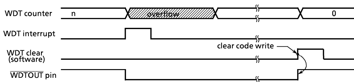
Figure 3.13 (2) Watchdog Timer Output During Overflow
