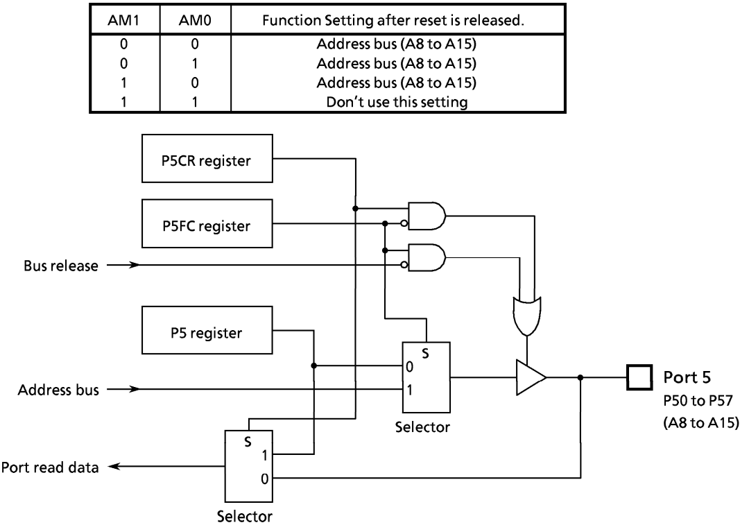
Figure 3.5 (6) Port 5
