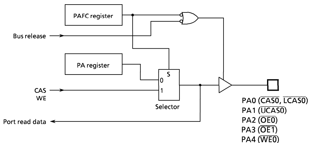
Figure 3.5 (10) Port A
