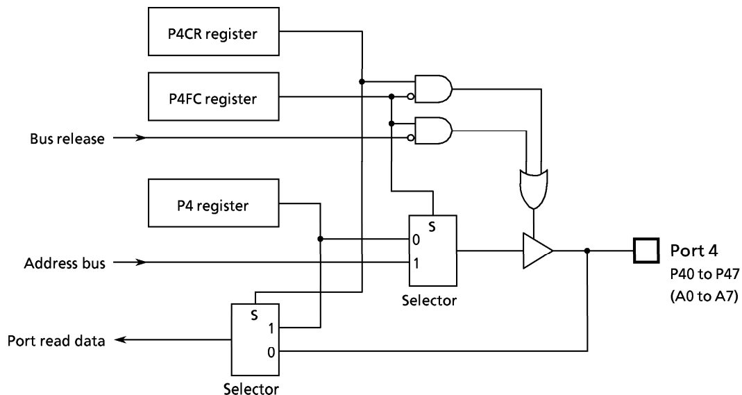
Figure 3.5 (5) Port 4
