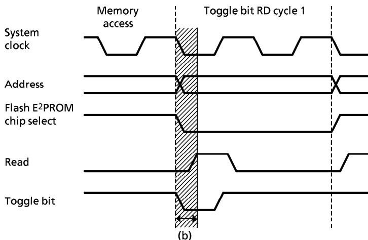
Figure 3.6 (3) Flash E 2 PROM Toggle Bit Read cycle
