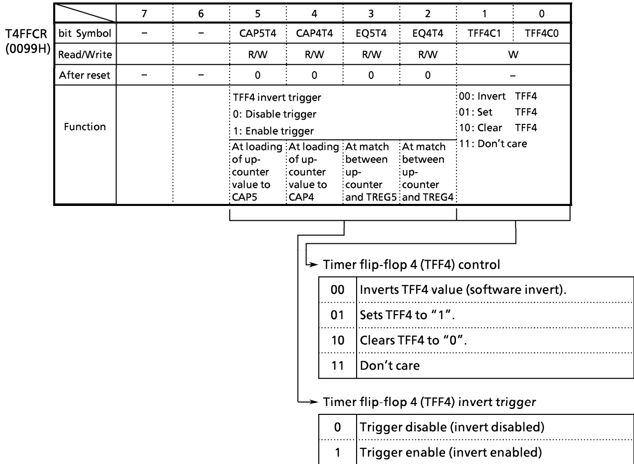
Figure 3.9 (7) 16-Bit Timer 4 F/F Control (T4FFCR)
