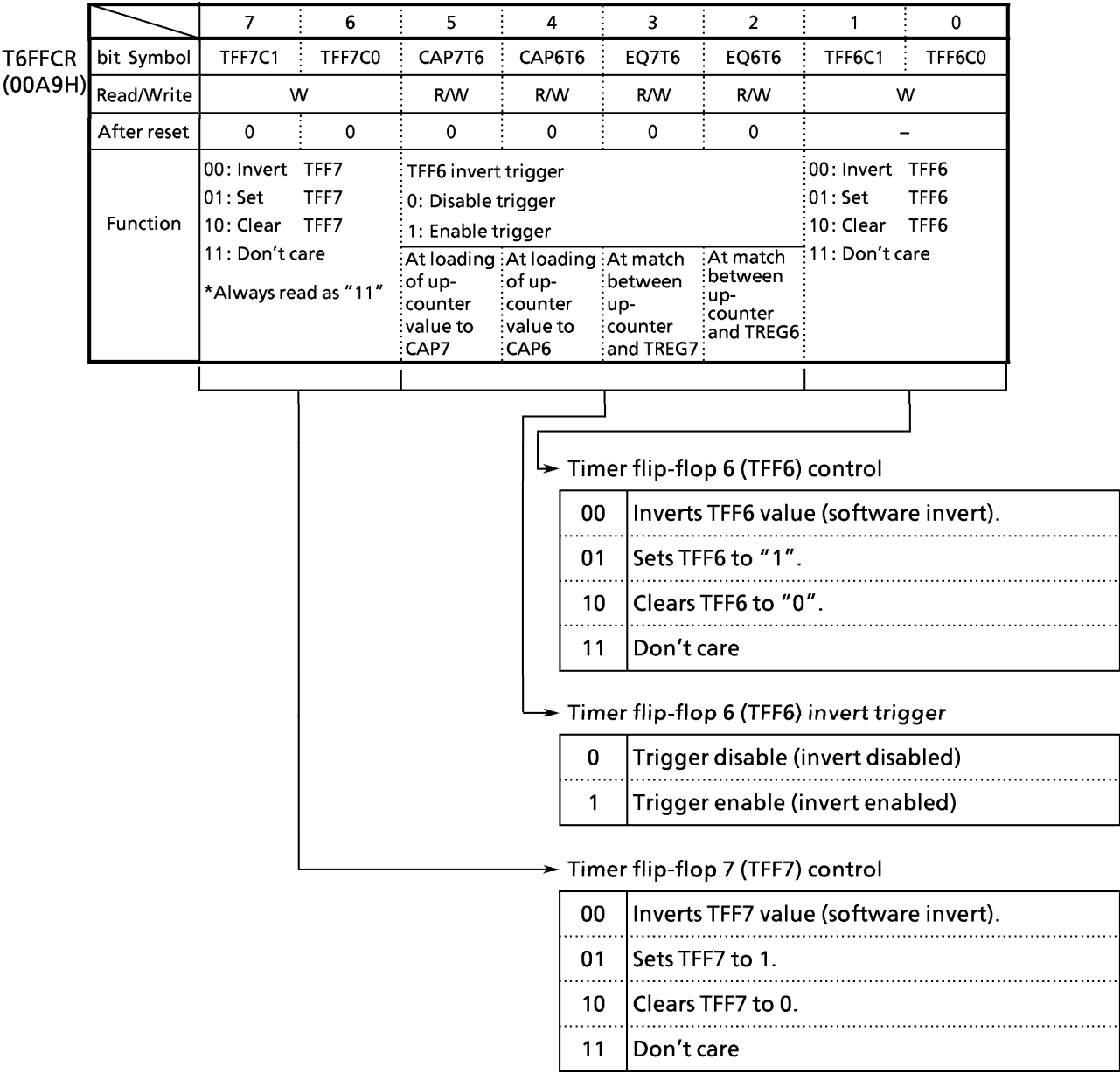
Figure 3.9 (10) 16-Bit Timer 6 F/F Control (T6FFCR)
