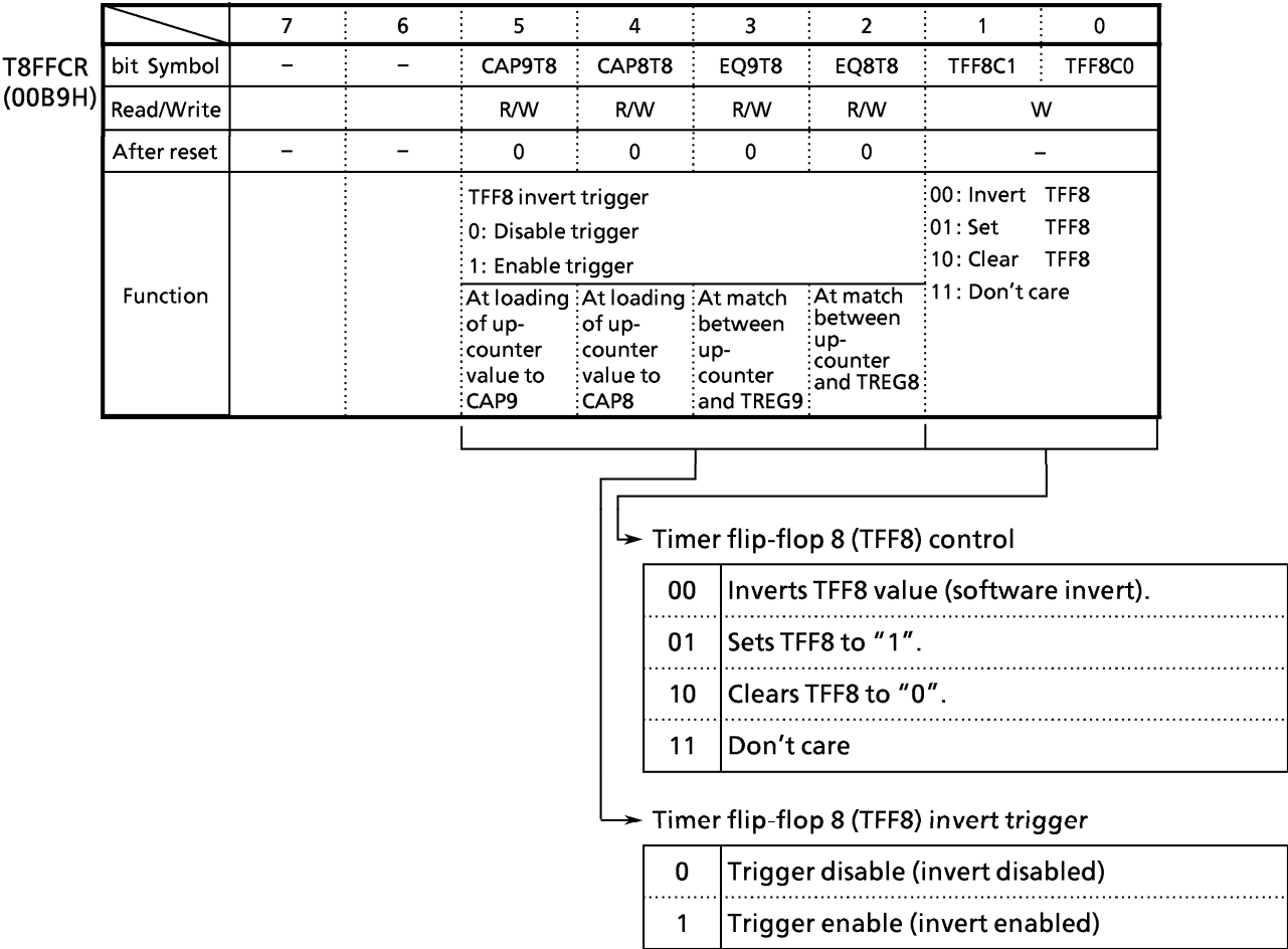
Figure 3.9 (13) 16-Bit Timer 8 F/F Control (T8FFCR)
