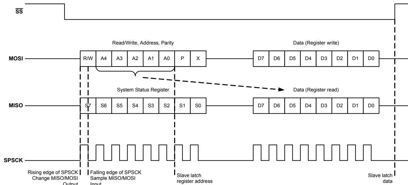
Figure 9. SPI Protocol
