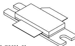
NI-780H-2L MMRF1009HR5
