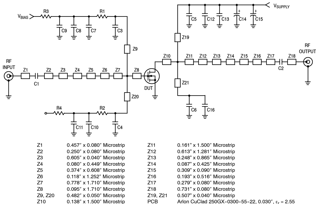
Figure 1. MMRF1009HR5(HSR5) Test Circuit Schematic
