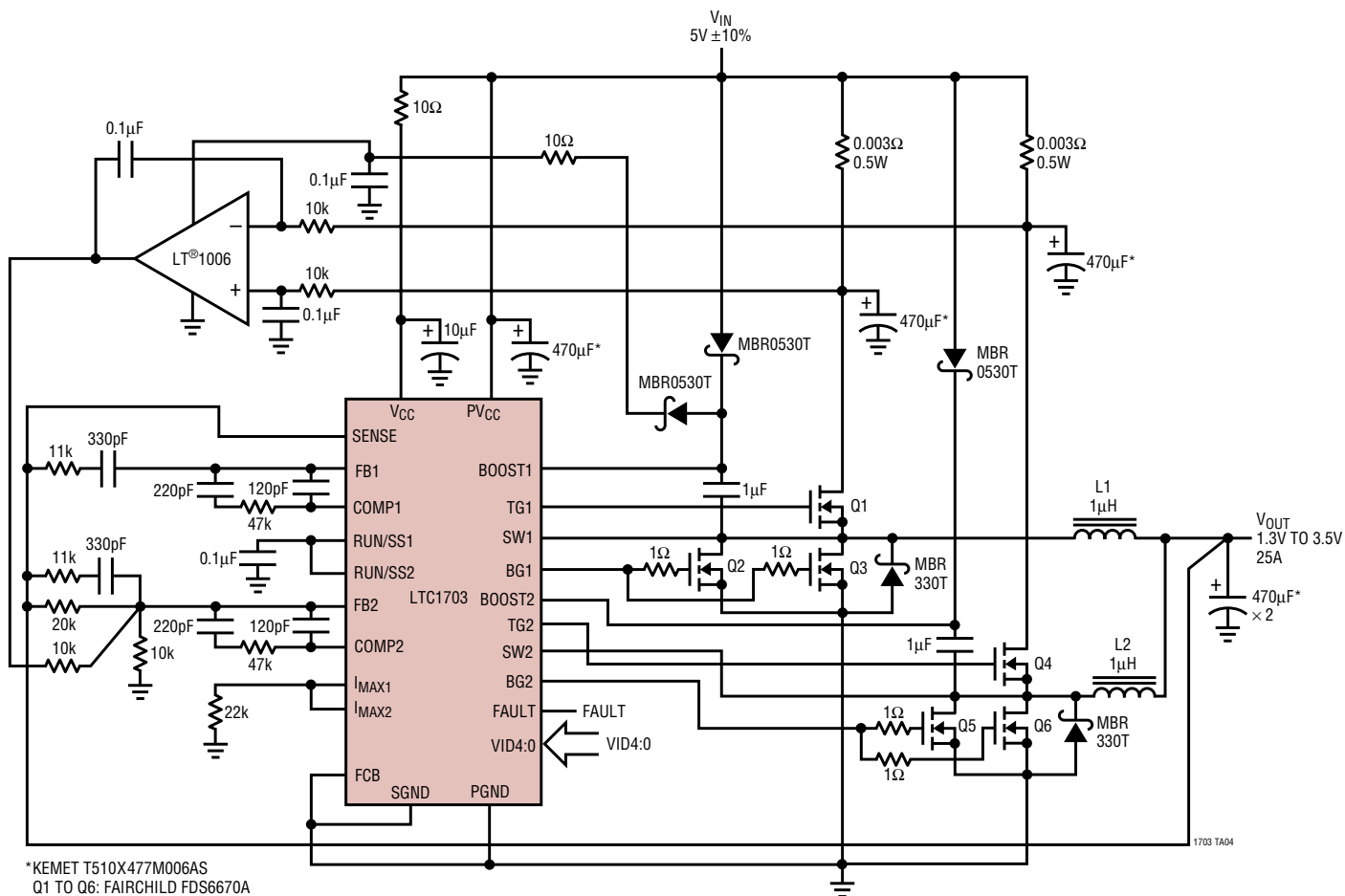
Single Output, 2-Phase, 25A VID Converter (V_{IN} = 5V, V_{OUT} = 0.9V \text{ to } 2.0V)
