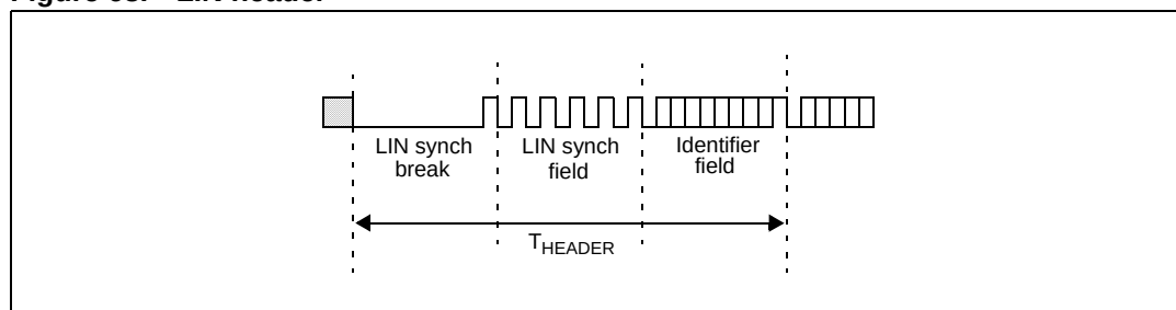
Figure 68. LIN header
