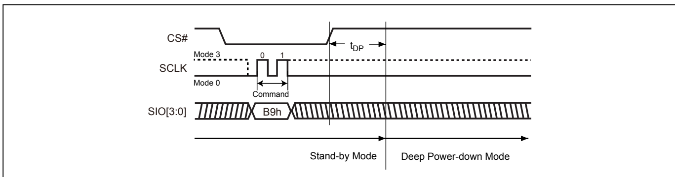
Figure 90. Deep Power-down (DP) Sequence (QPI Mode)
