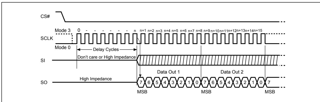
Figure 73. Fast Boot Sequence (QE=0)
