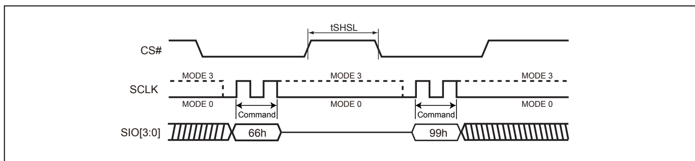
Figure 110. Reset Sequence (QPI mode)
