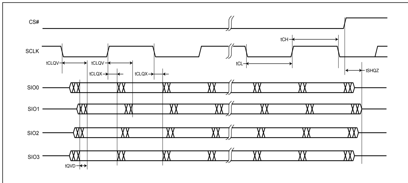
Figure 3. Output Timing
