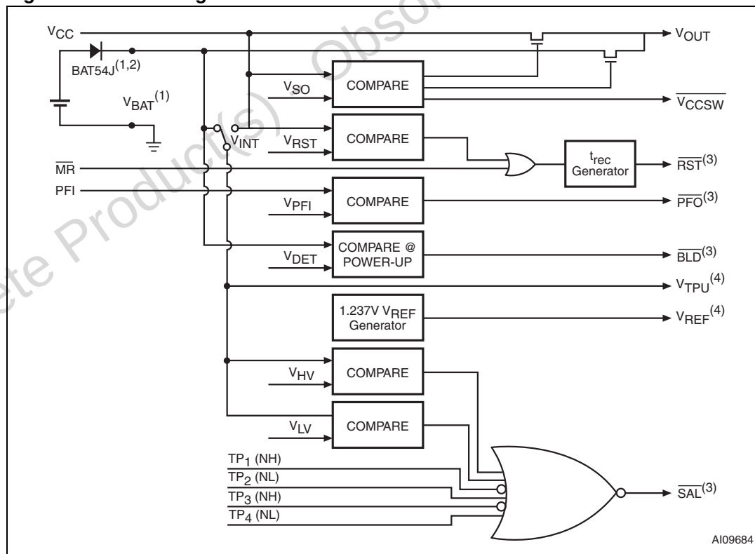
Figure 3. Block diagram
