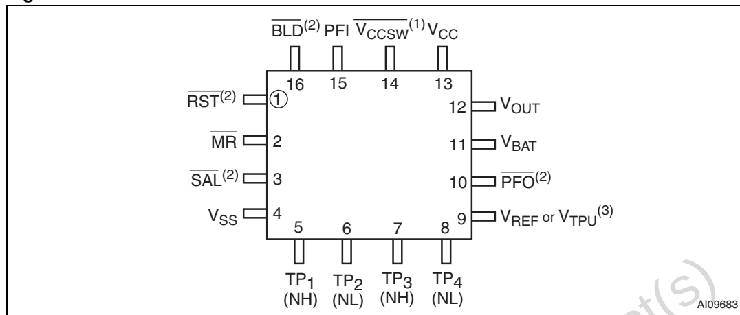
Figure 2. QFN16 connections
