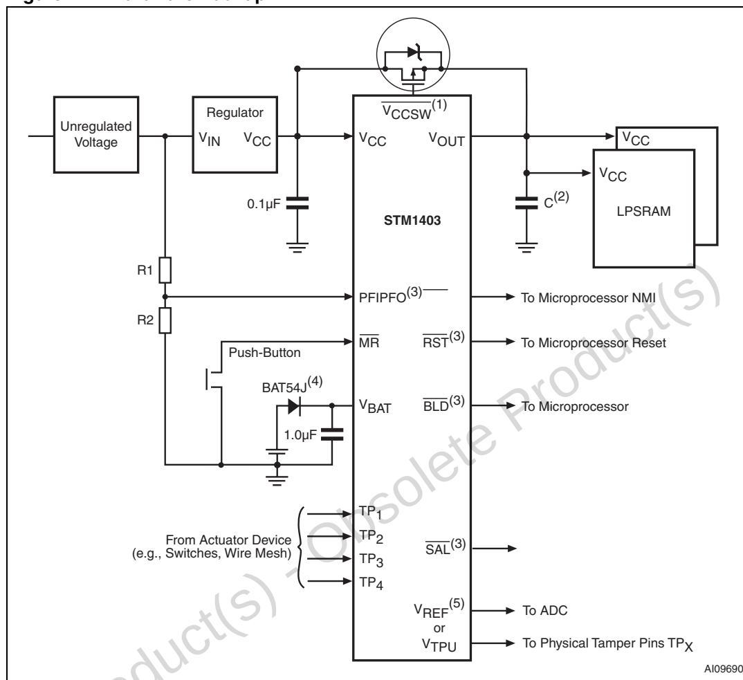
Figure 4. Hardware hookup
