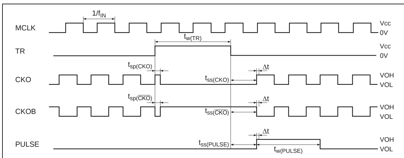
Figure 1 Trigger Mode 1
