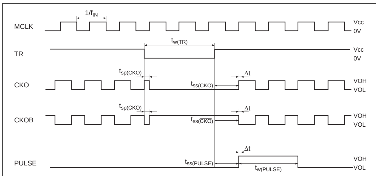
Figure 2 Trigger Mode 2
