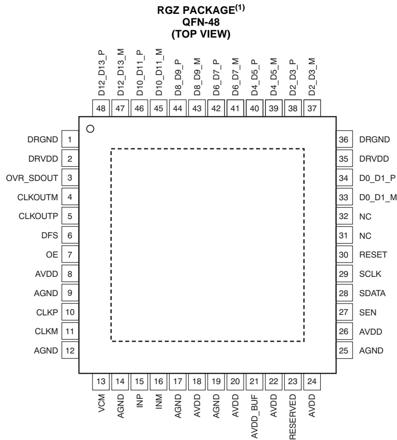
Figure 1. ADS41B49 LVDS Pinout
