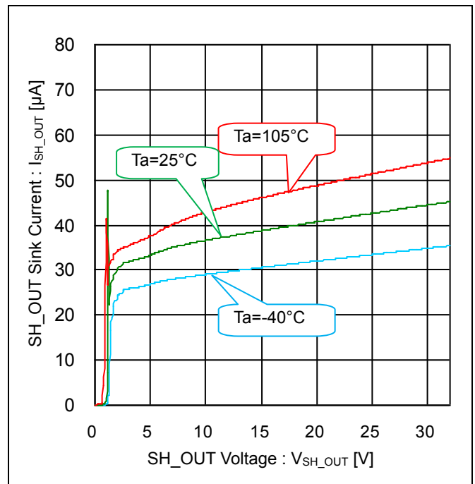
Figure 6. Circuit Current vs SH_OUT Voltage (V_SH_IN=0V)
