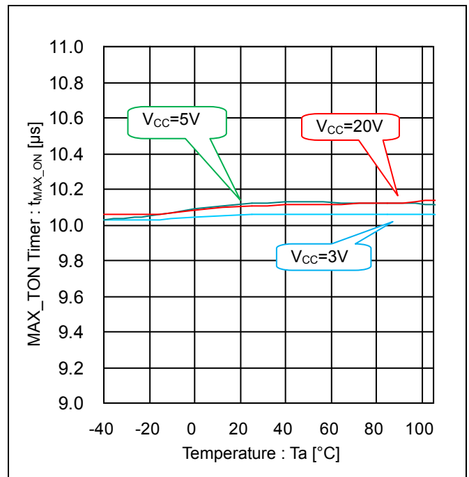
Figure 8. MAX_TON Timer vs Temperature ( R_{MAX\_TON}=100k\Omega , V_{DRAIN}=-0.3V \leftrightarrow V_{CC} \times 2 )
