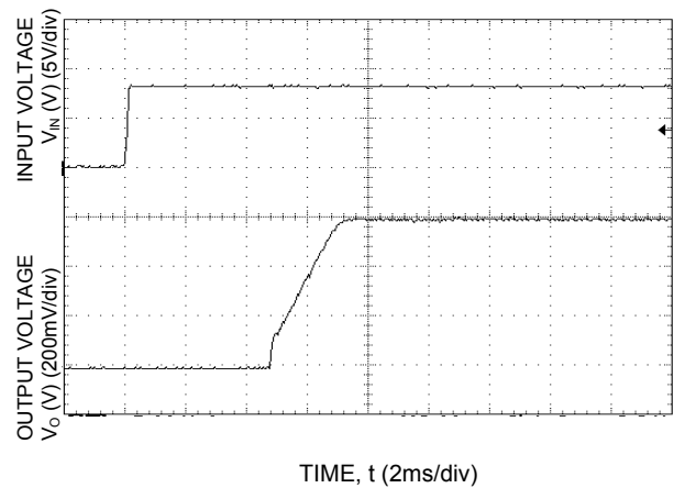
Figure 6. Typical Start-up Using Input Voltage ( V_{in}=8\text{V} , I_o=I_{o,max} ).
