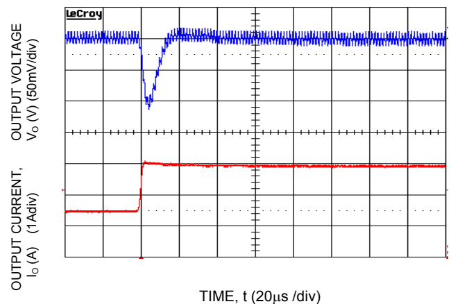
Figure 34. Transient Response to Dynamic Load Change from 50% to 100% at 12Vin, C_{out}=1x47\mu F , C_{Tune}=820pF & R_{Tune}=261
