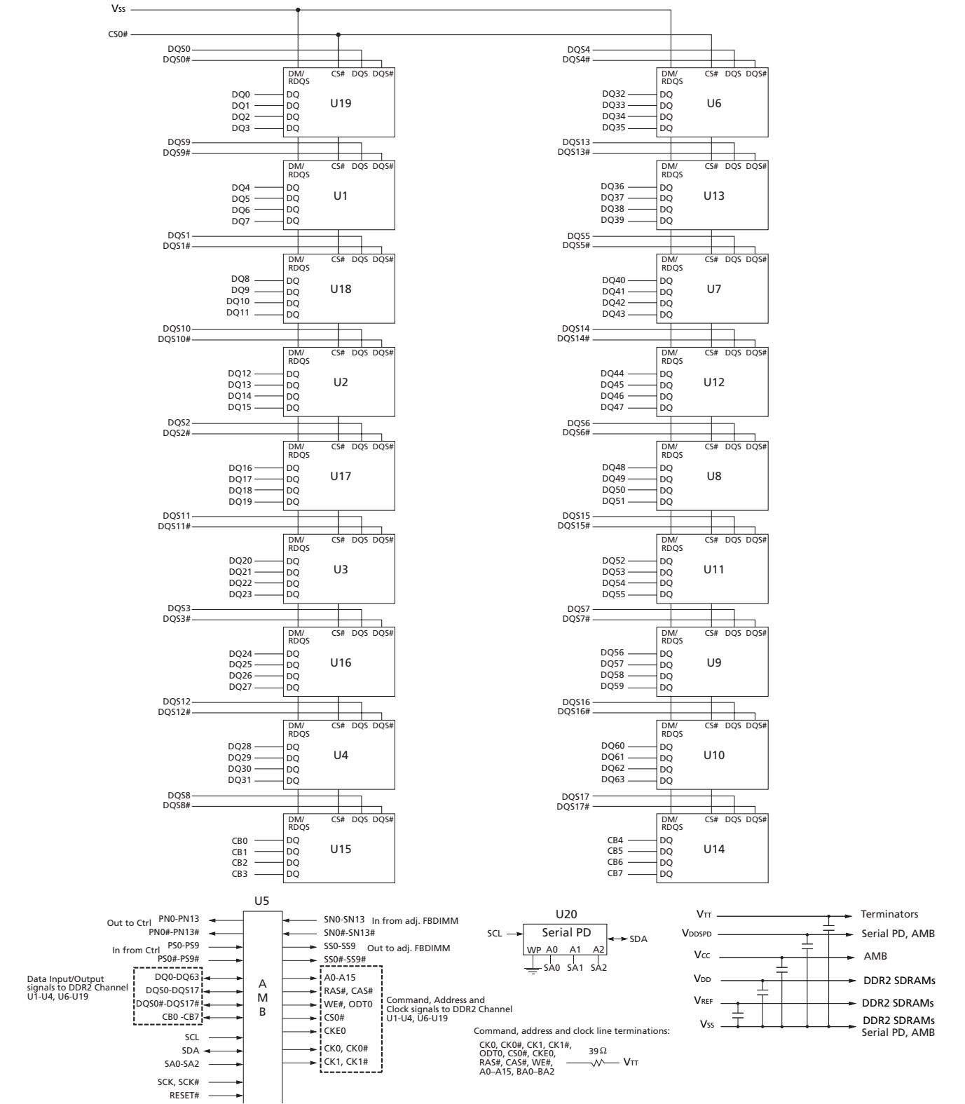
Figure 5: FBDIMM Functional Block Diagram
