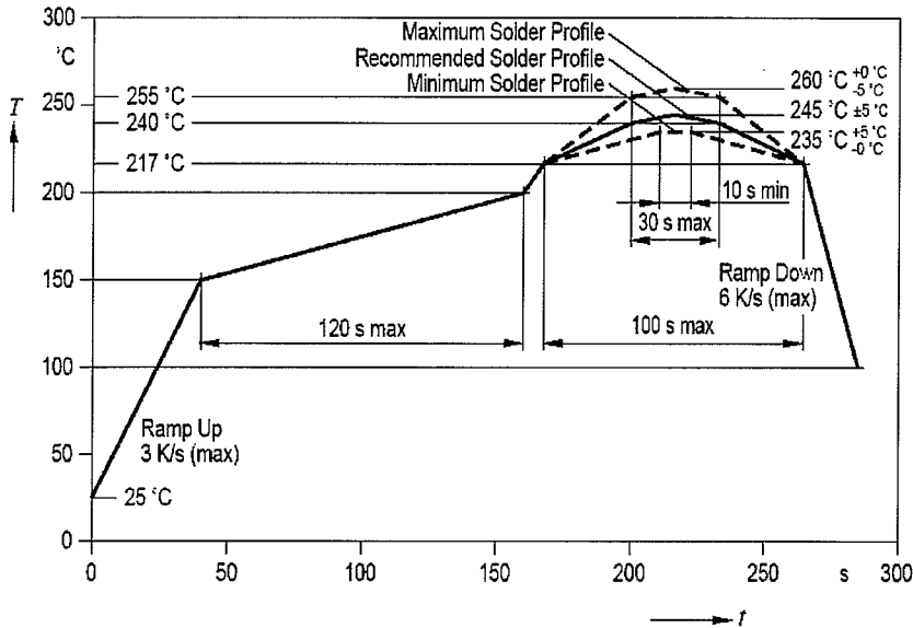
RoHS REFLOW PROFILE
