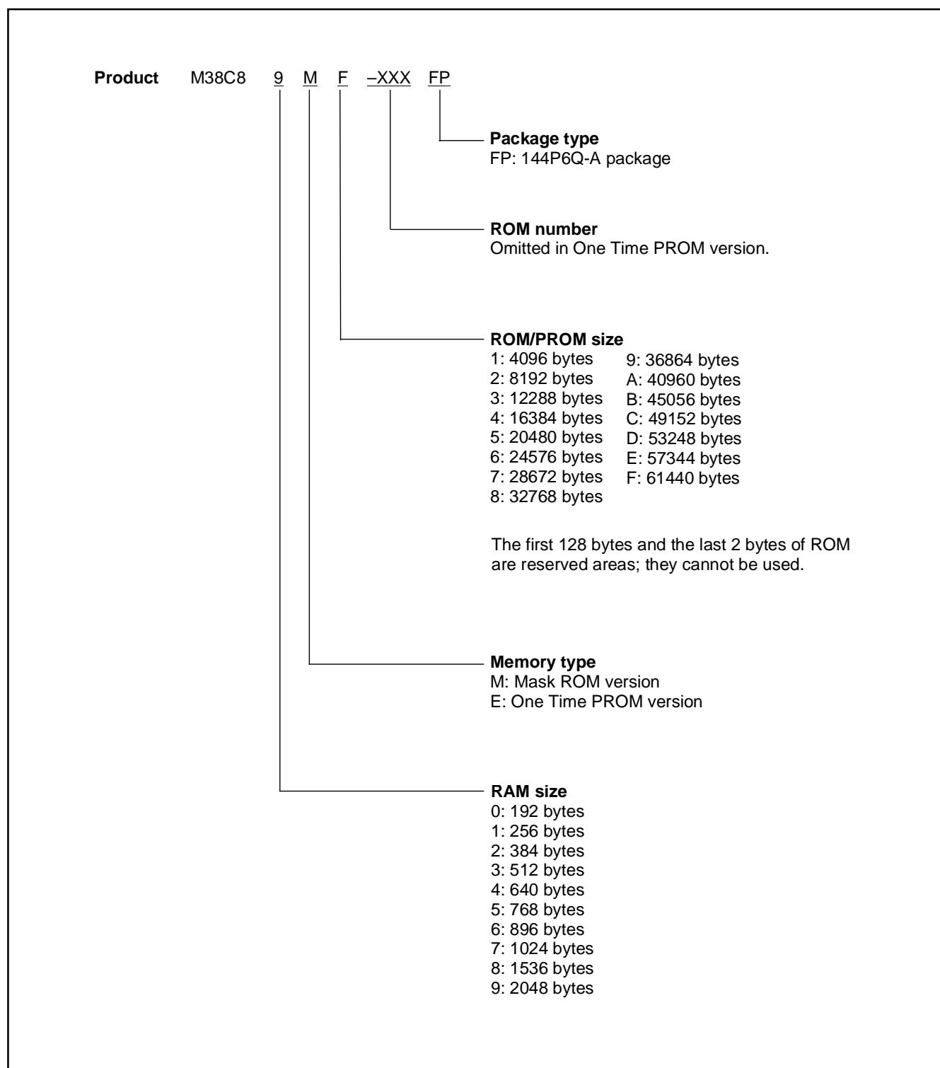
Fig. 3 Part numbering
