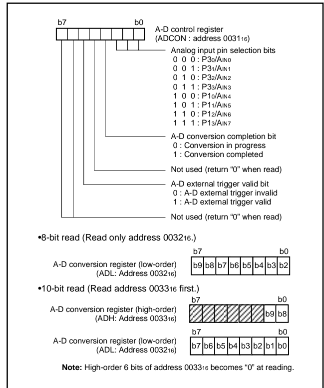
Fig. 25 Structure of A-D control register
