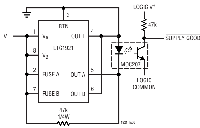
Single -48V Supply Monitor
