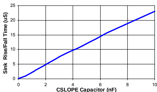
Typical CSLOPE vs Slope Times
