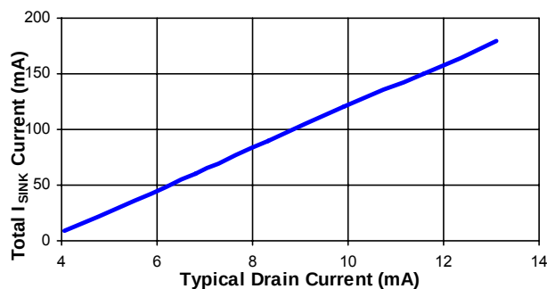
LX1991 Typical Drain Current Vs Sink Current
