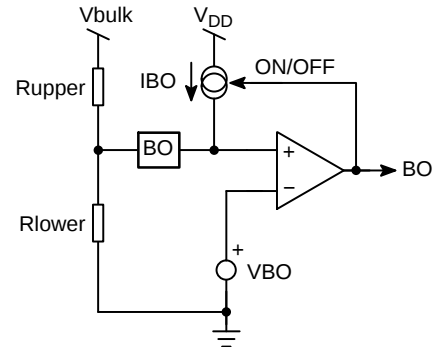
Figure 40. The Internal Brown-out Configuration with an Offset Current Source
