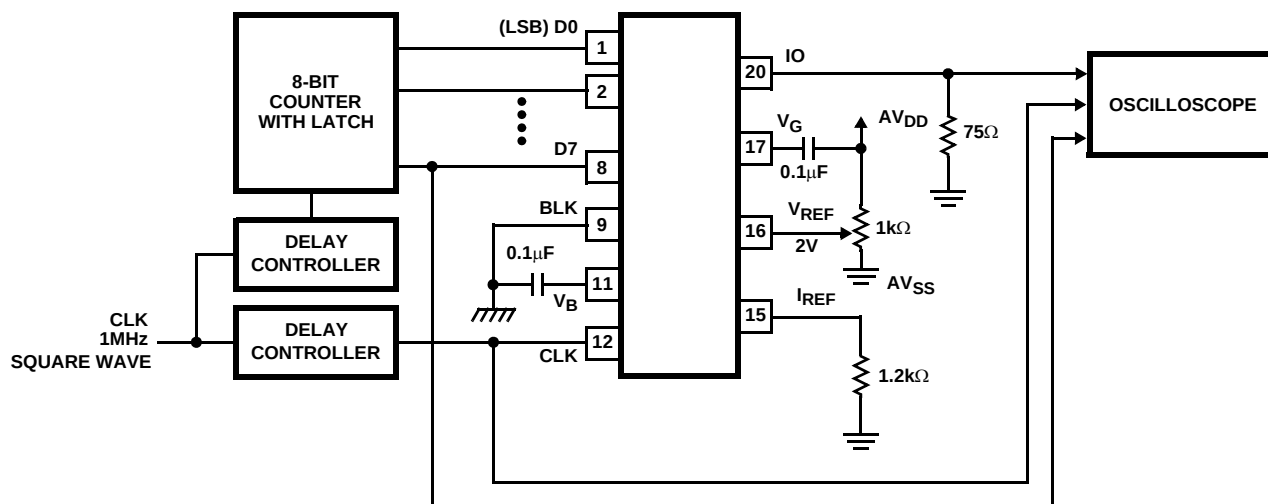
FIGURE 8. SET UP HOLD TIME AND GLITCH ENERGY TEST CIRCUIT
