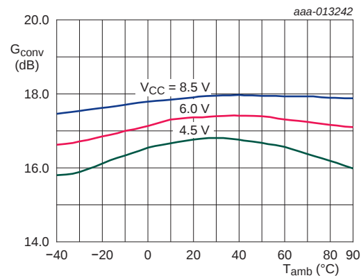
Fig 10. Conversion gain versus temperature
