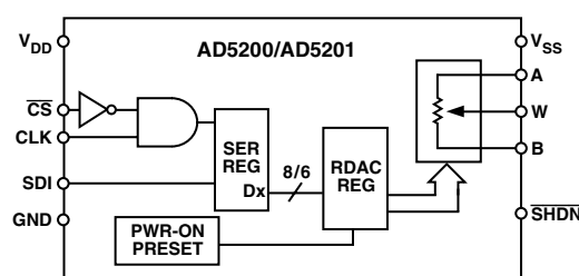
Figure 3. Block Diagram
