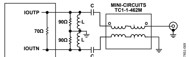
Figure 68. Recommended Mix Mode Configuration Offering Extended RF Bandwidth Using a TC1-1-462M Balun
