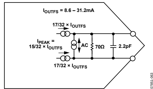
Figure 62. Equivalent DAC Output Circuit
