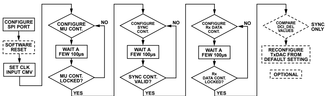
Figure 74. Flowchart for Initialization and Configuration of the AD9739
