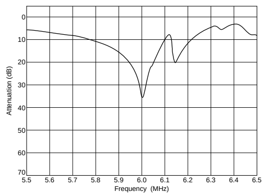
TPSRF6M00J00-B0
