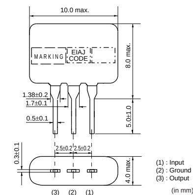
CDSRF_CK Series
