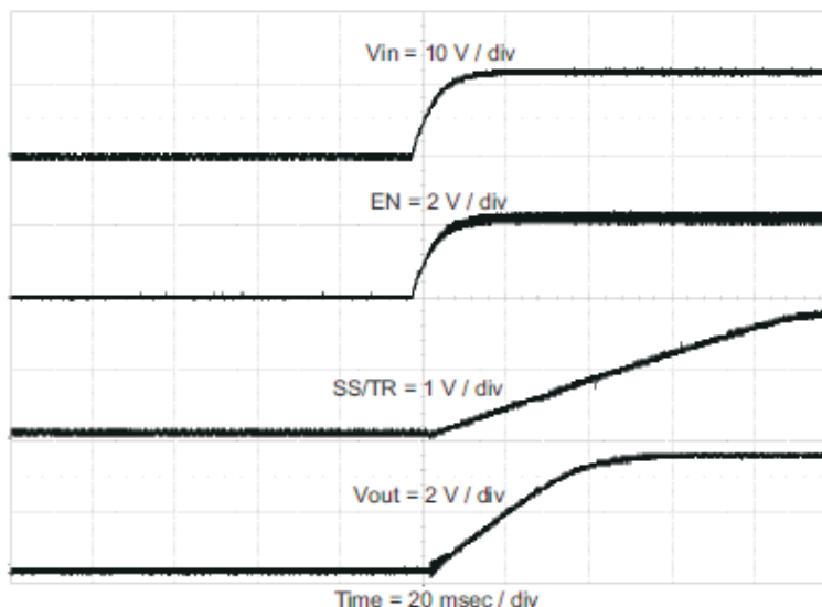
Figure 2-9. TPS54620EVM-374 Start-Up Relative to V_{IN}
