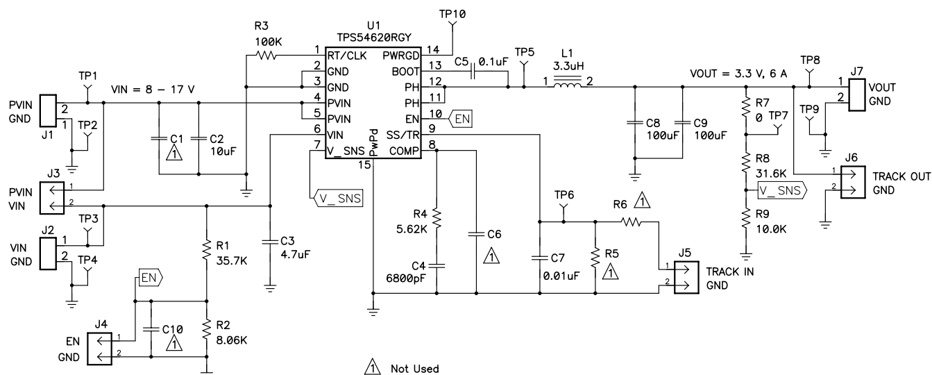
Figure 4-1. TPS54620EVM-374 Schematic
