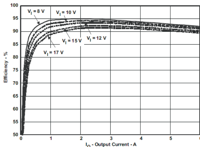
Figure 2-1. TPS54620EVM-374 Efficiency
