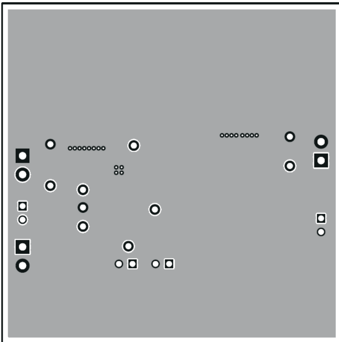
Figure 3-2. TPS54620EVM-374 Layout 2
