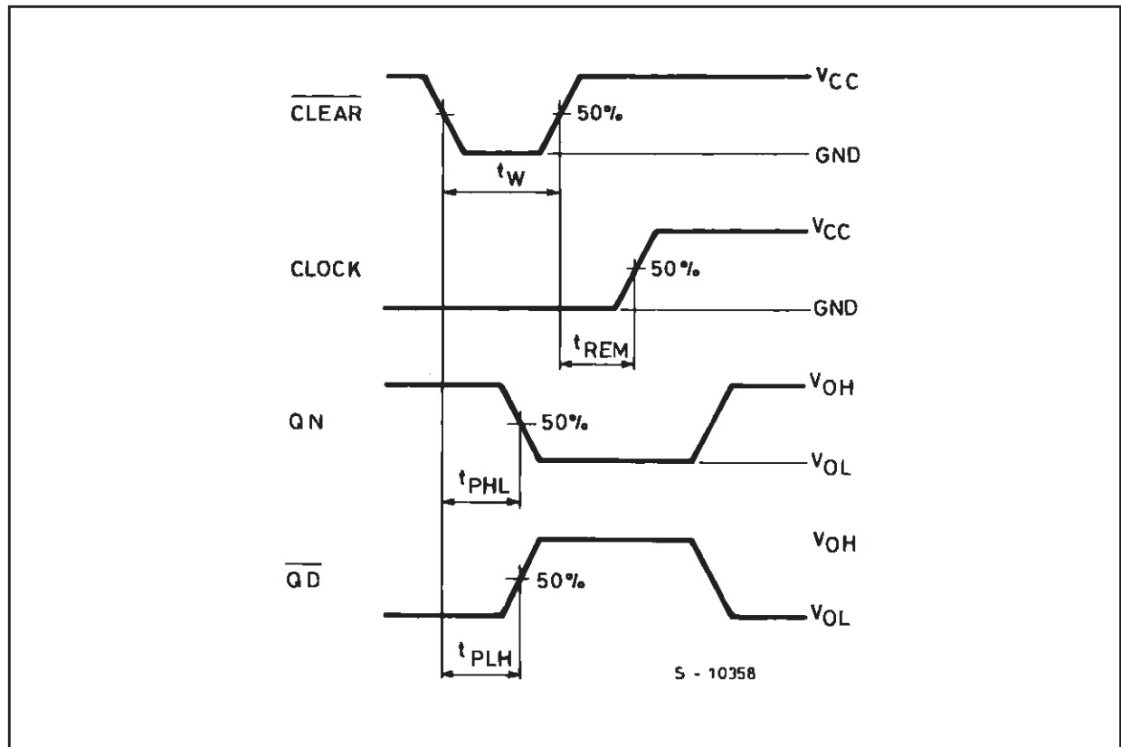
WAVEFORM 2 : MINIMUM PULSE WIDTH AND REMOVAL TIME ( f=1\text{MHz} ; 50% duty cycle)
