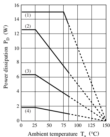
P_D - T_a (AN77xx series)
