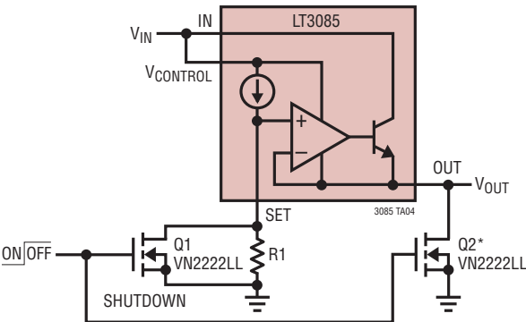
Adding Shutdown
