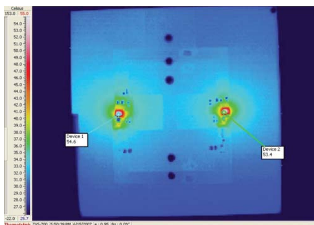
Figure 5. Temperature Rise at 800\text{mW} Dissipation
