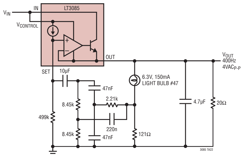
Power Oscillator
