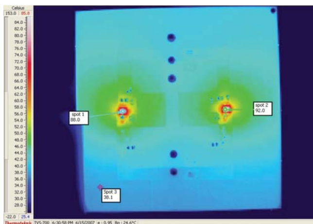
Figure 6. Temperature Rise at 1.7\text{W} Dissipation
