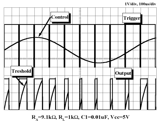
Figure 10. Waveforms of Pulse Width Modulation
