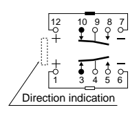
2 coil latching (Reset condition)
