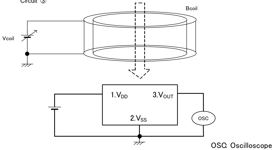
Circuit ③
