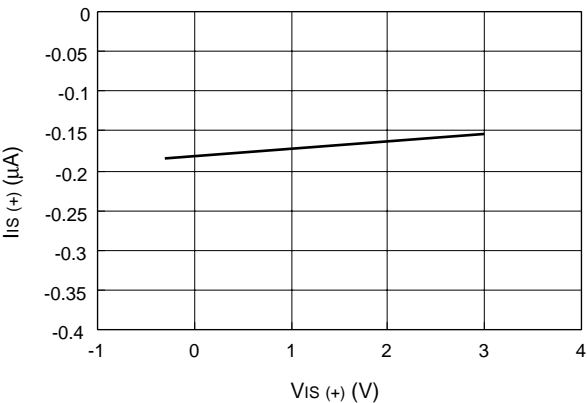
IS (+) pin current (I IS (+)) vs. IS (+) pin voltage (V IS (+)) FA5510/11
