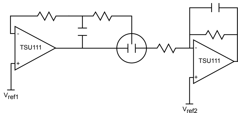
Figure 37. Potentiostat schematic using the TSU111
