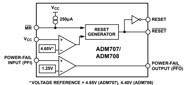
Figure 2. ADM707/ADM708
