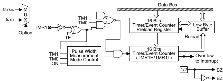
Timer/Event Counter 1
