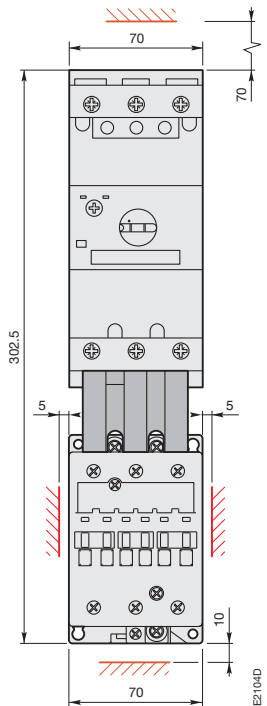
MS 49x + BEA 75/495 + A 50, A 63, A 75
