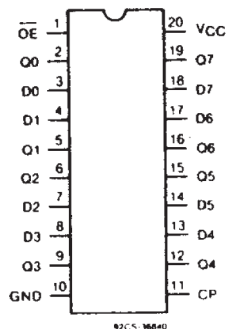
Figure 3-1. CDx4AC/ACT374, CD74AC534
