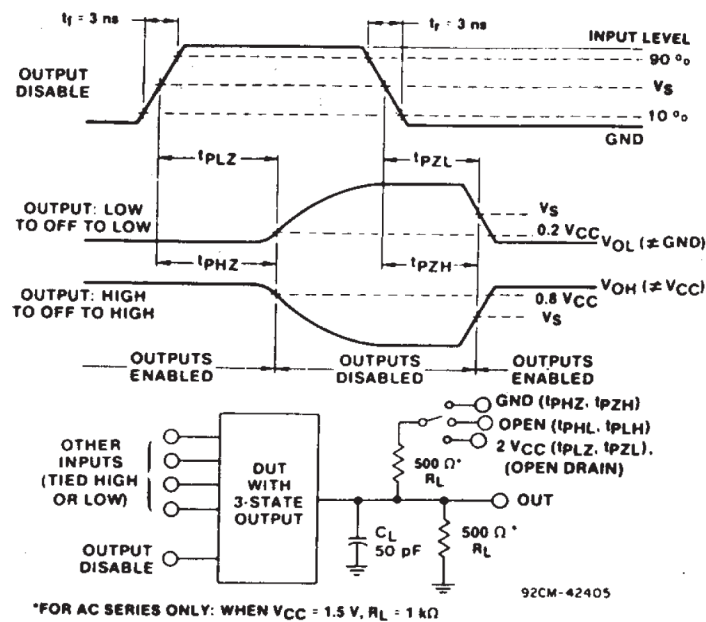
Figure 5-1. Simultaneous Switching Transient Waveforms.
