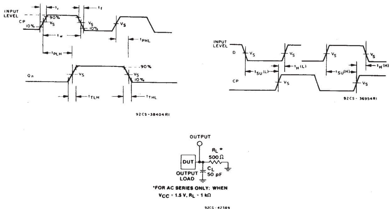
Figure 5-3. Propagation Delay Times and Test Circuit.
