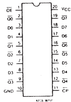
Figure 3-2. CDx4AC/ACT374, CD74AC534
