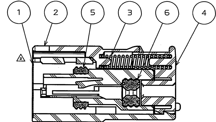
SECT. A-A
