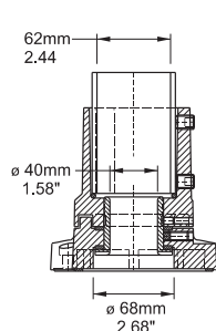
Front Section
