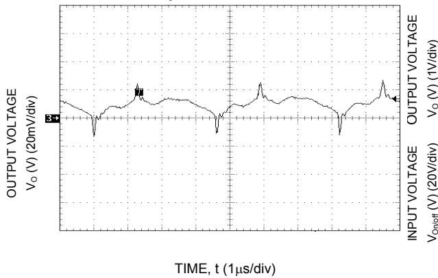
Figure 2. Typical Output Ripple and Noise (Vin = 48Vdc, I_o = 25A).
