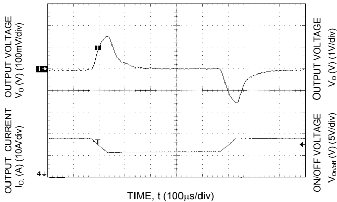
Figure 3. Typical Transient Response to Dynamic Load change Load from 50% to 75% to 50% of Full load at 48 Vdc Input.
